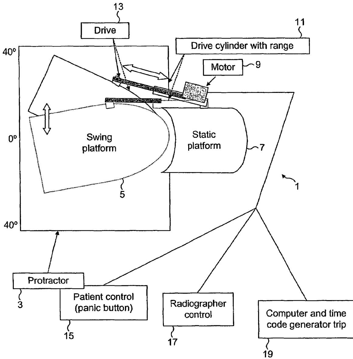
Passive Motion Platform - Top Elevation
